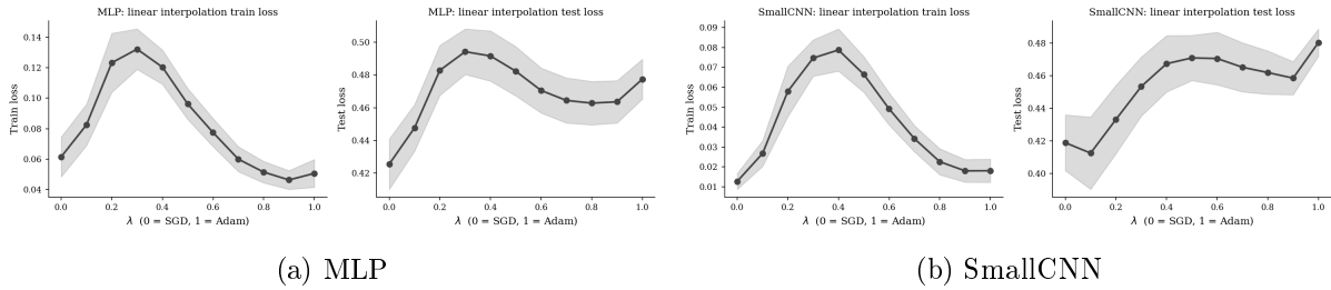
Figure 14: Linear mode connectivity: training and test loss along \theta(\lambda) = (1 - \lambda)\theta_{\text{SGD}} + \lambda\theta_{\text{Adam}} , with BatchNorm recalibrated at interior \lambda . Solid line is mean over five matched seeds; band is \pm 1 std.
