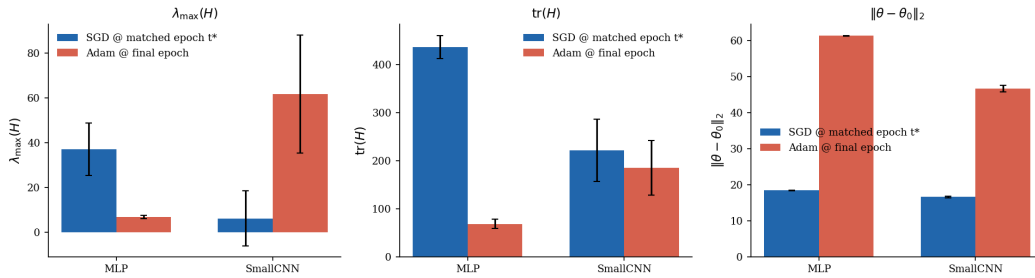
Figure 17: Loss-matched geometry comparison across both architectures, summarizing \|\theta - \theta_0\|_2 , \lambda_{\text{max}}(H) , \text{tr}(H) and function-space disagreement.
