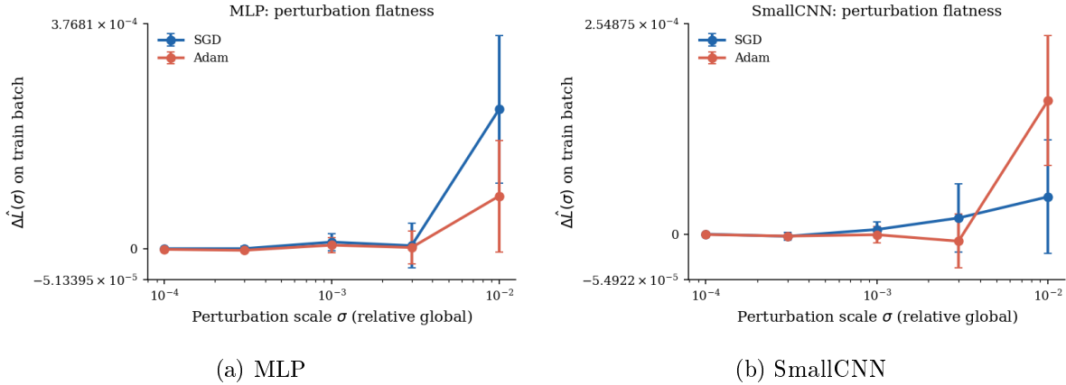
Figure 13: Mean training-loss increase \Delta \widehat{L}(\sigma) under relative isotropic Gaussian perturbations, averaged over five matched seeds and K = 10 perturbations per \sigma . Values at \sigma \leq 3 \times 10^{-3} are at the noise floor ( \leq 10^{-5} ); the operational comparison is at \sigma = 10^{-2} .
