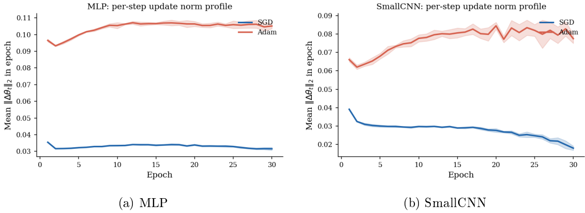
Figure 12: Mean per-step update norm \overline{\|\Delta\theta_t\|_2} by epoch, five matched seeds.
