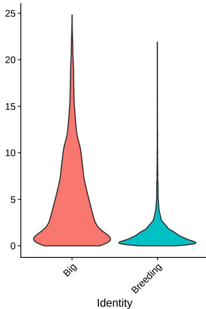
percent.mt
