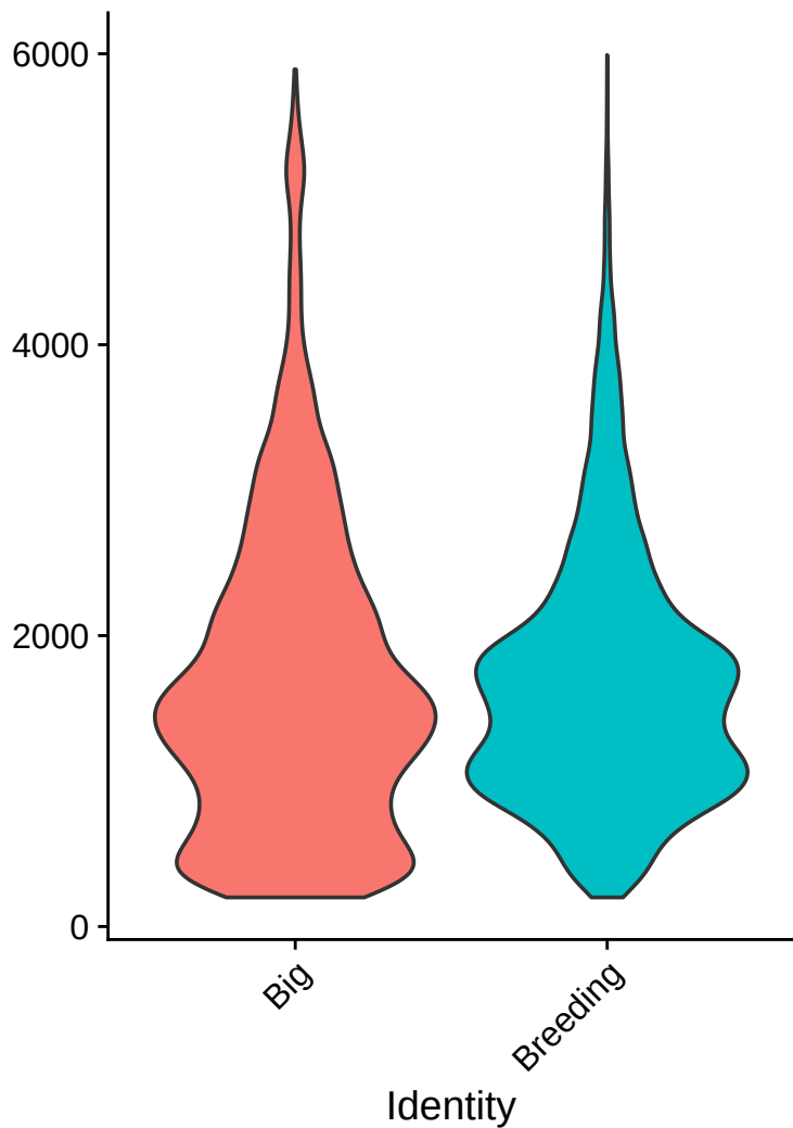
nFeature_RNA
