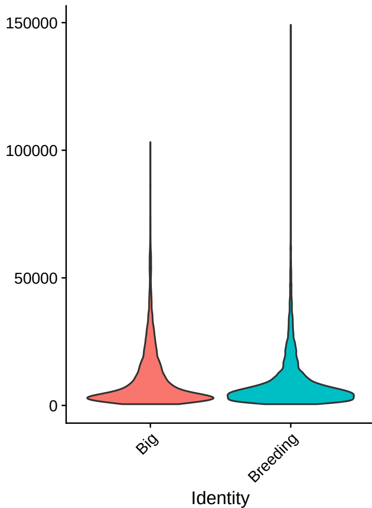
nCount_RNA
