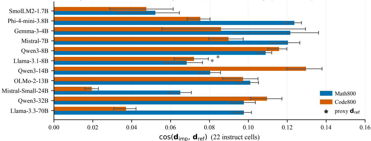
(a) Recognition \perp Refusal — 22 main-grid cells (mean cos 0.087, range [0.019, 0.130])
