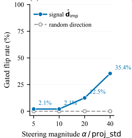
(b) Mistral-7B / code800 A→U (L15)
