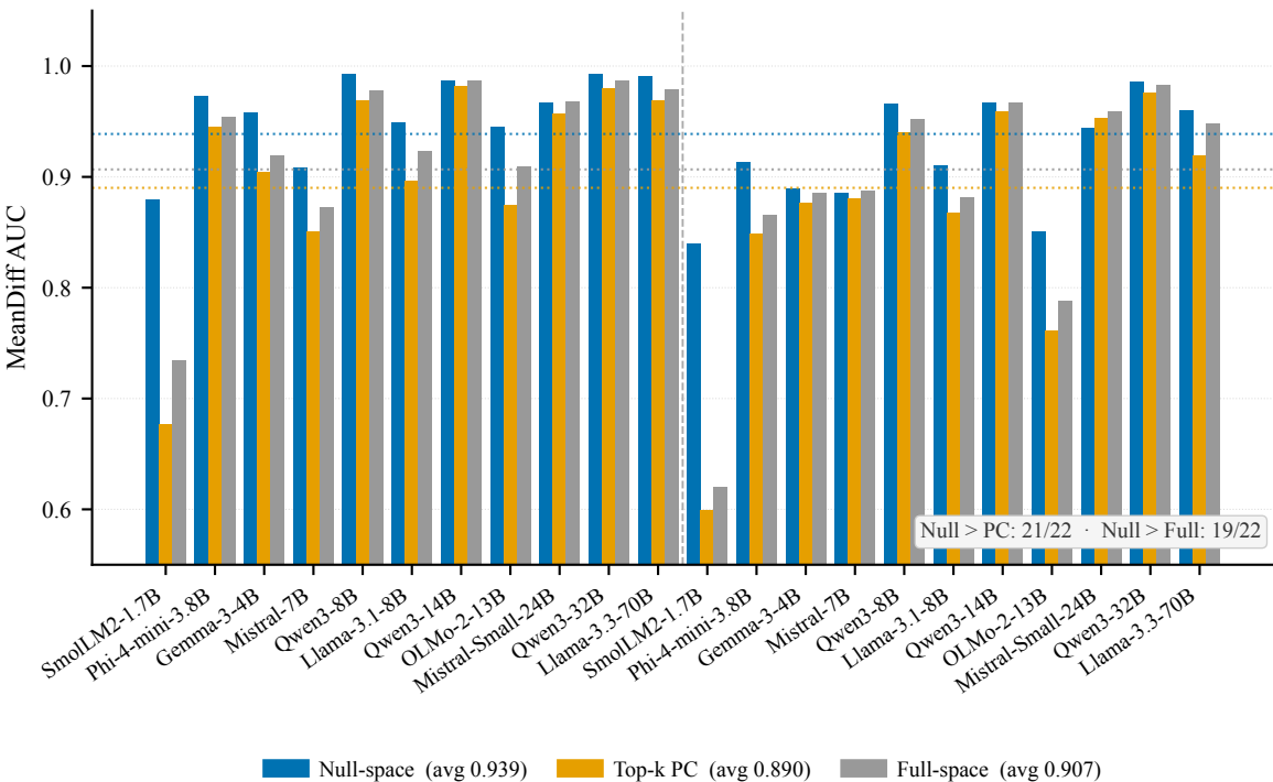
Projection ablation (MeanDiff AUC, 5-seed avg, 22 cells) Math800 Code800
