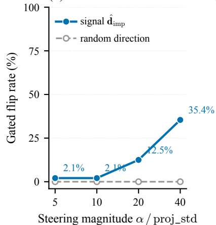
(b) Mistral-7B / code800 A \rightarrow U (L15)
