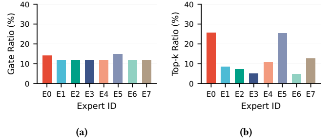
Figure 6: Expert routing statistics of the MoE on DeHate : (a) the distribution measured by gate probability ratio. (b) the distribution of experts measured by top- k selection ratio.
