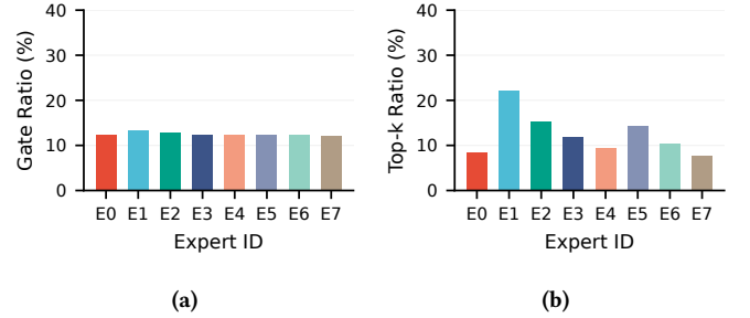
Figure 5: Expert routing statistics of the MoE on MHC_EN : (a) the distribution measured by gate probability ratio. (b) the distribution of experts measured by top- k selection ratio.
