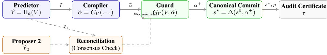
Figure 3: MemPatch Parameter-Free Runtime Flow. Compatibility Mode is shown as the main execution path: predictions flow from the predictor to the compiler, Revision Guard, and canonical commit, yielding an audit certificate. Consensus Mode operates as an optional branch with deterministic reconciliation under multiple proposers.
