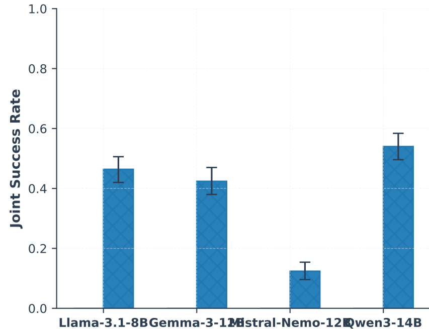
(a) Joint Revision Success Rate (95% CI)
