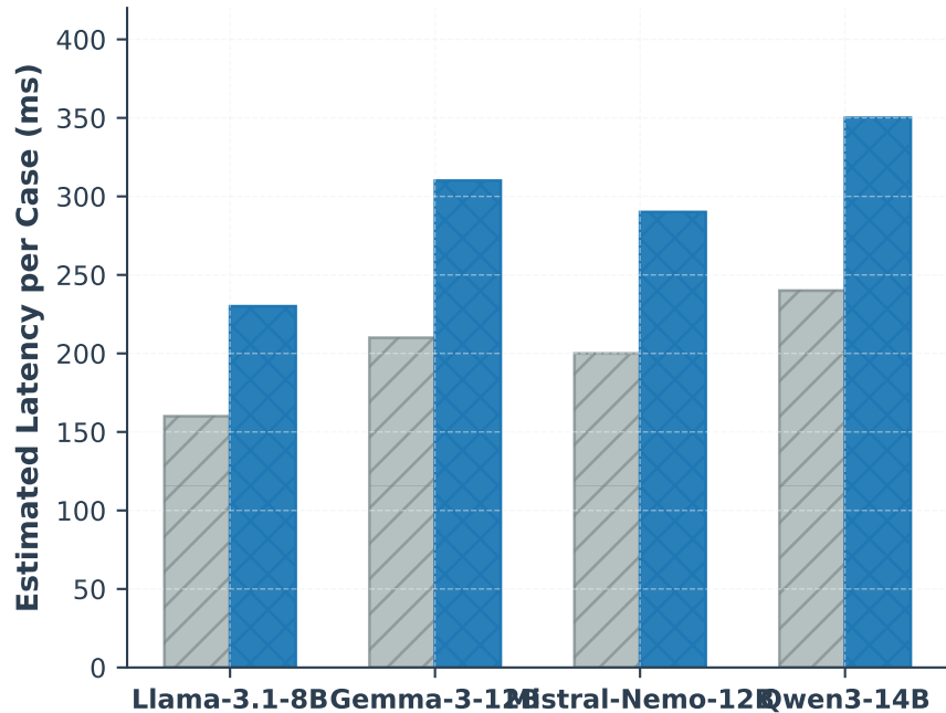
(b) Estimated Inference Latency
