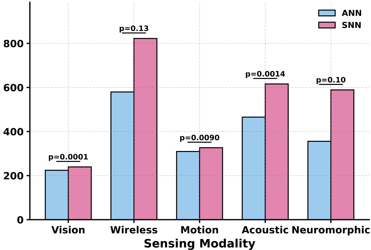
Average Peak Memory Footprint (MB)
