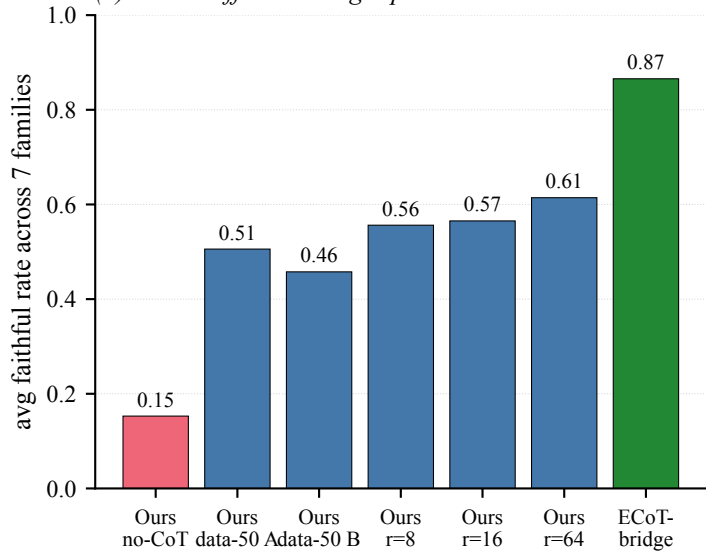
(b) Causal effect — huge spread
