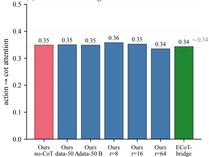
(a) Attention on CoT segment — all similar
