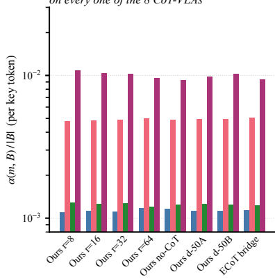
(c) Per-token: instruction beats CoT by 3.7–4.2× on every one of the 8 CoT-VLAs
