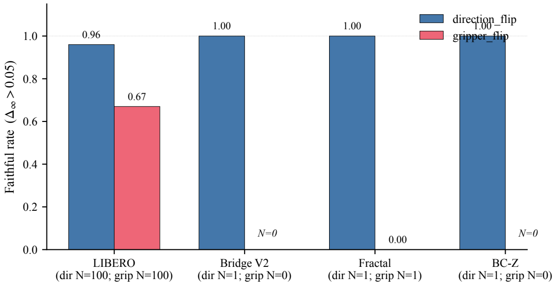
ECoT-bridge causal-edit pilot (N=1 per non-LIBERO corpus)
