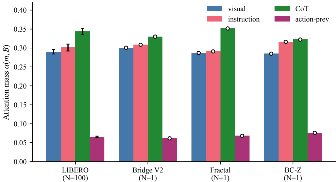
ECoT-bridge attention across 4 corpora (LIBERO mean \pm std; N=1 pilot elsewhere, open circles)
