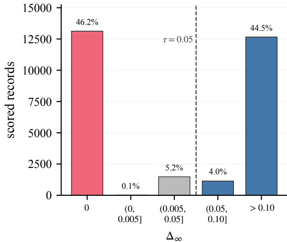
(a) 28,443 records: 46% are exactly zero
