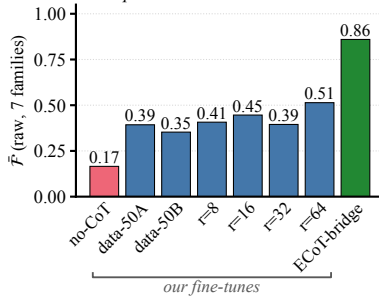
(b) Causal effect, raw: 5.2 \times spread
