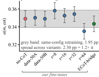
(a) Attention on CoT: spread \approx retraining noise
