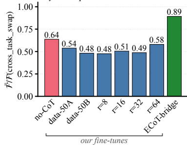
(c) Ceiling-normalized: only 1.9 \times spread
