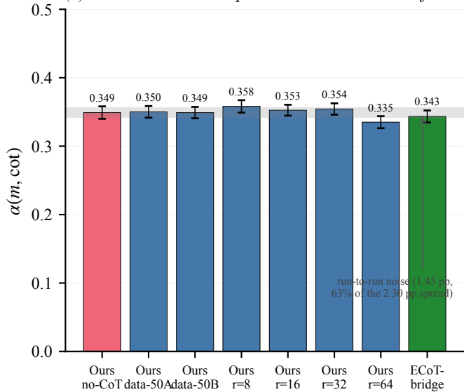
(a) Attention on CoT: spread is inside the noise floor
