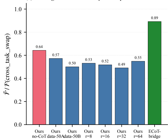
(c) Ceiling-normalized: only 1.8 \times spread
