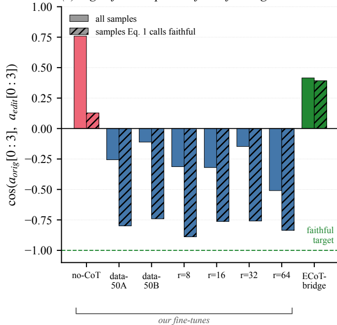
(b) Sign of the response after left \leftrightarrow right is reversed
