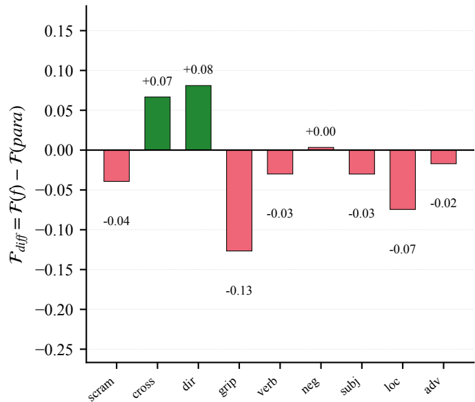
(c) ours-no-cot: differential leaderboard (paraphrase floor = 0.19)
