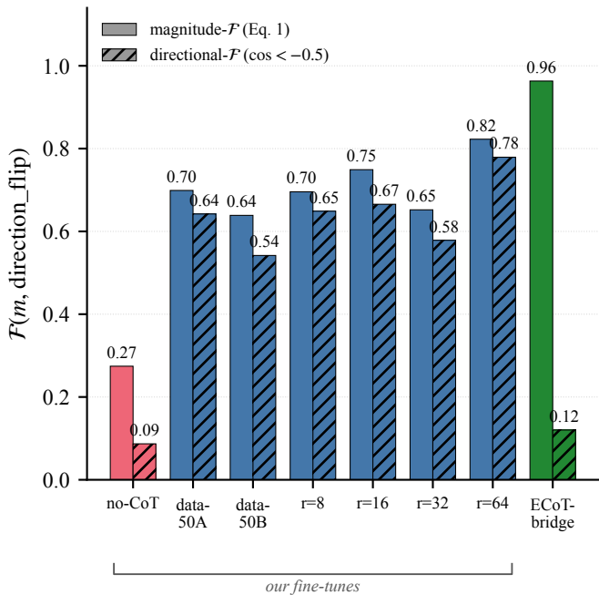
(a) The flagship edit: magnitude vs direction
