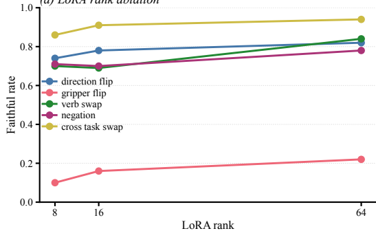
(a) LoRA rank ablation
