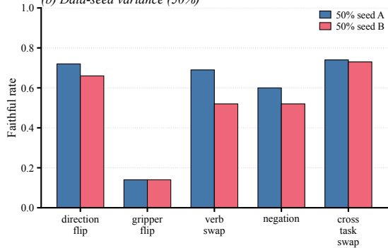
(b) Data-seed variance (50%)
