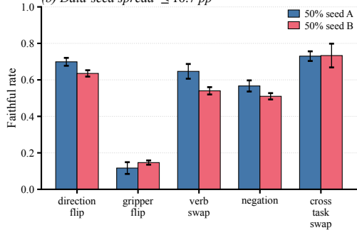
(b) Data-seed spread \leq 10.7 pp
