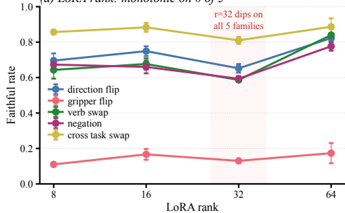
(a) LoRA rank: monotonic on 0 of 5
