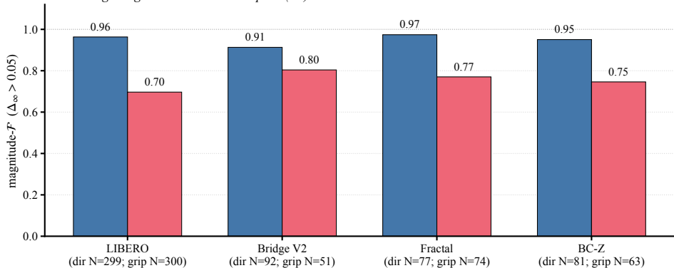
ECoT-bridge magnitude- \mathcal{F} across 4 corpora (F5)
