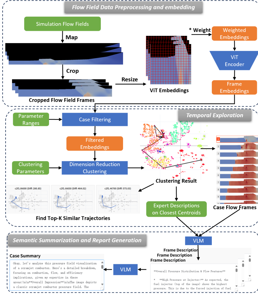
Fig. 1 Overview of TemporalFlowViz , including preprocessing and embedding of flow fields, temporal trajectory-based exploration, and semantic summarization and report generation via expert-informed vision-language modeling.
