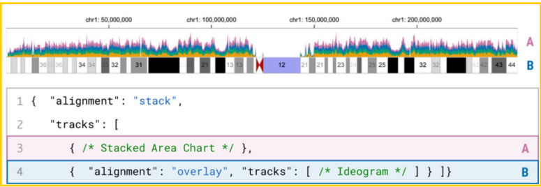
Fig. 6. Track Alignment. Tracks can be either stacked or overlaid. The ability to nest multiple tracks with different alignment options allows flexible track composition. This figure shows an area chart that is juxtaposed with an ideogram (i.e., overlaid tracks).
