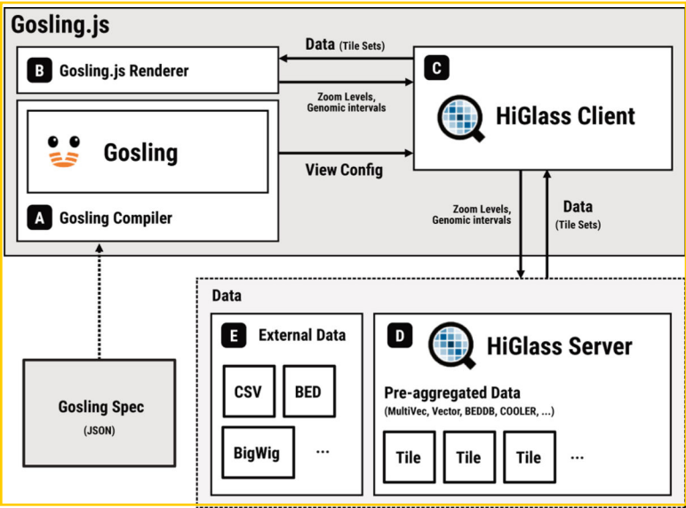
Fig. 11. System Structure of Gosling.js. Gosling.js consists of three main components: (A) a compiler, (B) a renderer, and (C) a HiGlass client [34].
