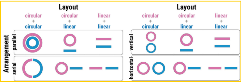
Fig. 8. View Arrangement. Four arrangement options used in different layouts cover broad arrangement of views (pink and blue).
