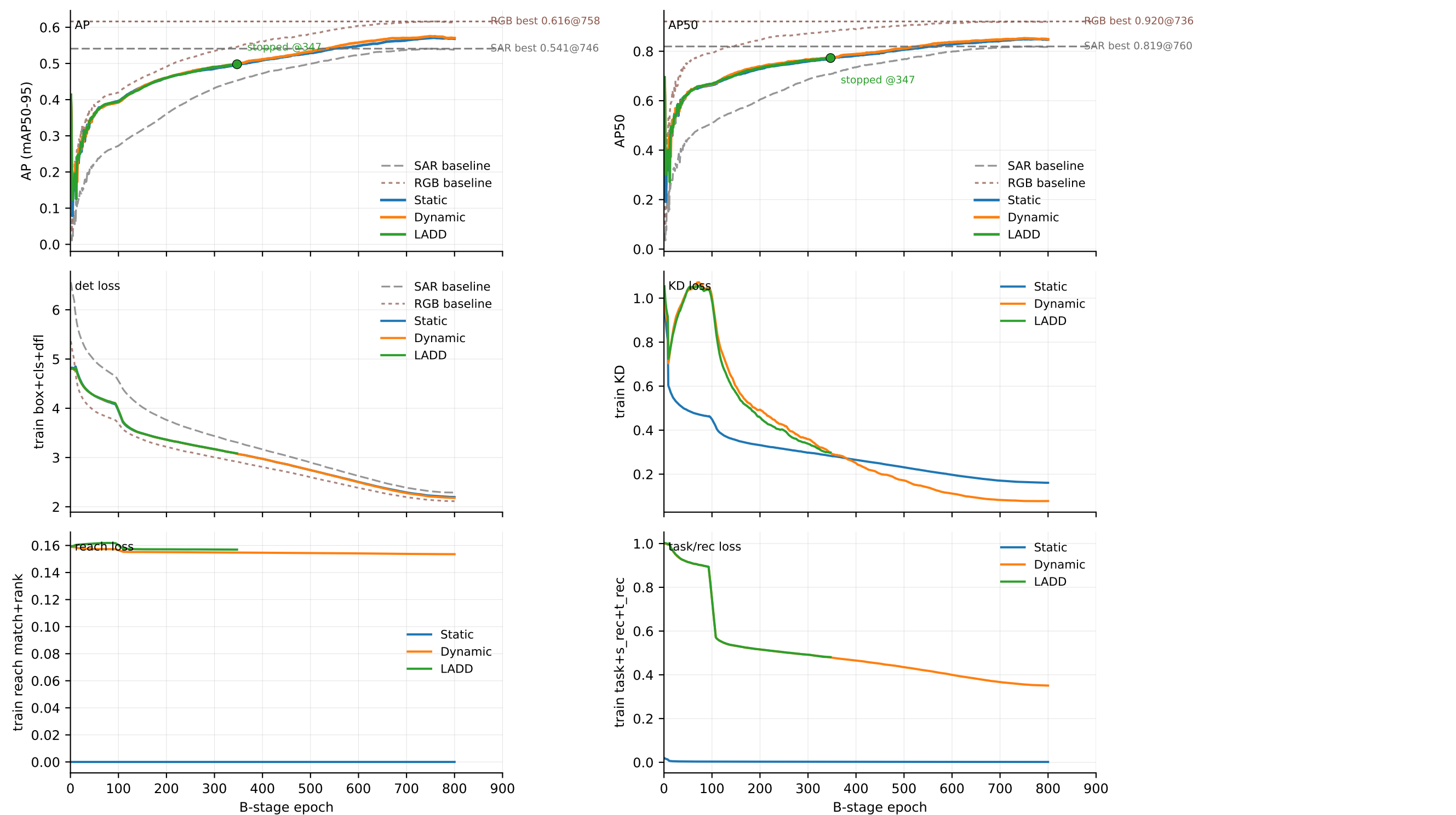
YOLO11n mosaic100 protocol. Thin dashed/dotted curves: same-capacity SAR/RGB baselines; horizontal lines: their best AP. LADD is the 4090 run interrupted at epoch 347; the green curve is short because the experiment has not been resumed.
