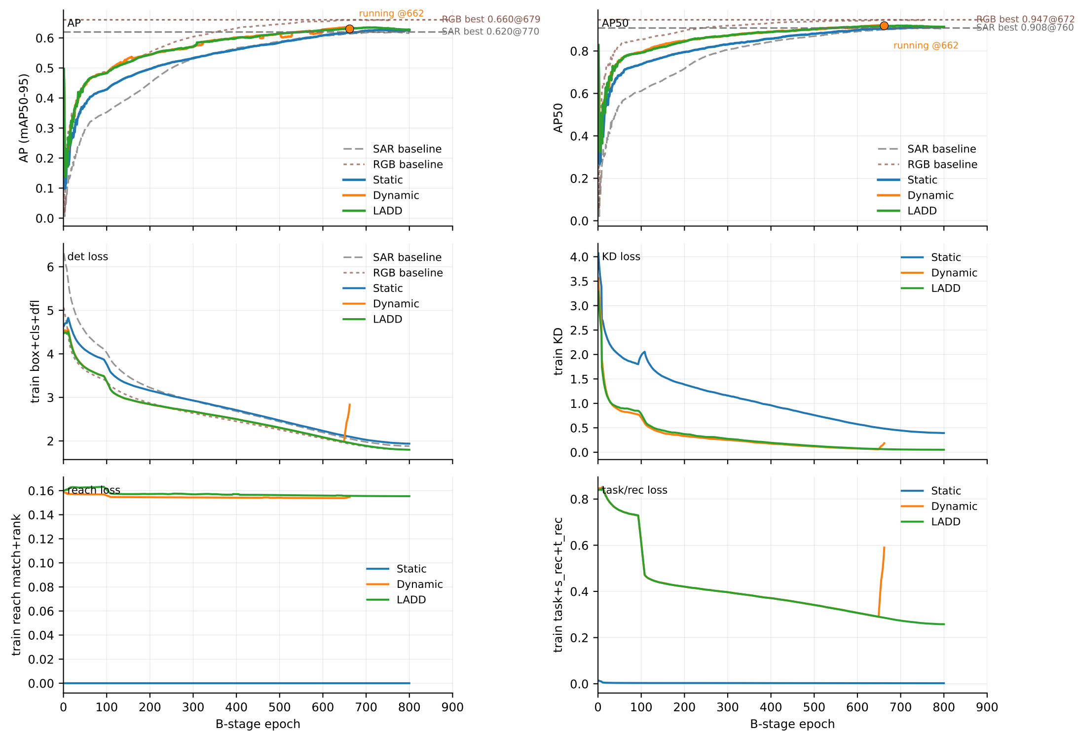
YOLO11s mosaic100 protocol. Thin dashed/dotted curves: same-capacity SAR/RGB baselines; horizontal lines: their best AP. Static and LADD are completed. Dynamic was resumed on 4090 and is shown up to the latest synced epoch.
