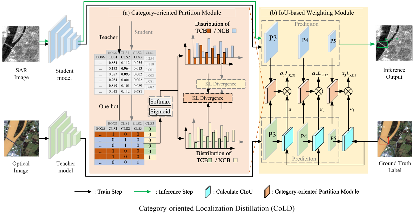
Fig. 2. Overall framework of our CoLD, where TCB denotes target category bounding boxes and NCB denotes nontarget category bounding boxes. A prior knowledge of the optical images is introduced using a specially designed CPM, and candidate bounding boxes with rich knowledge are obtained. An IWM then adaptively focuses on high-quality candidate bounding boxes in the teacher network based on the corresponding IoU score. Finally, only SAR images are input for inference. (a) CPM. (b) IWM.
