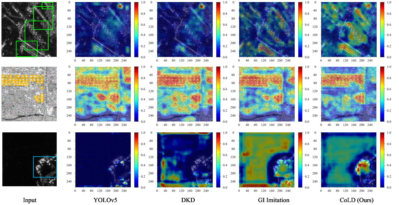
Fig. 6. Visualization of the learning attention map using GradCAM. The results show that our method allows for a better focus on the position of the object and has very little background noise. The SAR object detection method cannot effectively focus on the location of the oil tanks without the guidance of optical images. Cross-modal methods do not take full advantage of the information in optical images, resulting in the introduction of more background noise.
