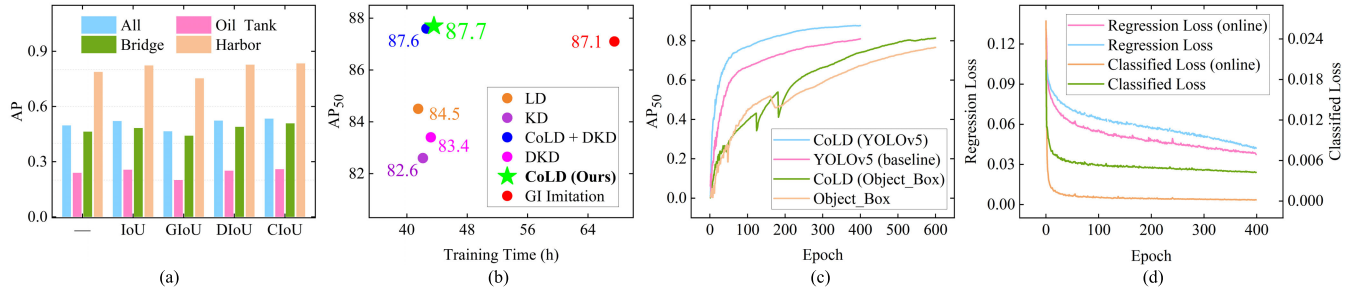
Fig. 7. (a) Performance comparison of using different IoUs (e.g., IoU, CIoU, DIoU, or GIoU) in IWM. (b) Training time (h) versus accuracy ( AP_{50} ) on OGSOD-1.0. The figure shows the accuracy and training time for each method. (c) Performance of CoLD in different methods. The results show that our method is strongly generalizable. (d) Performance comparison between online and offline distillation. The results show that online distillation allows the network to converge faster and gives lower loss values.
