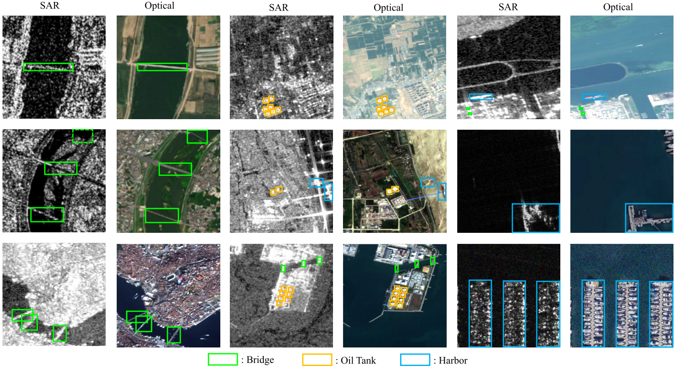
Fig. 3. Visualization of optical and SAR image pairs in OGSOD-1.0, where bridges, harbors, and oil tanks are indicated by green, blue, and yellow boxes, respectively. Despite using static objects for annotation, images from various time periods still include missing objects (e.g., the green dashed box in the SAR image), revealing our dataset is more challenging.
