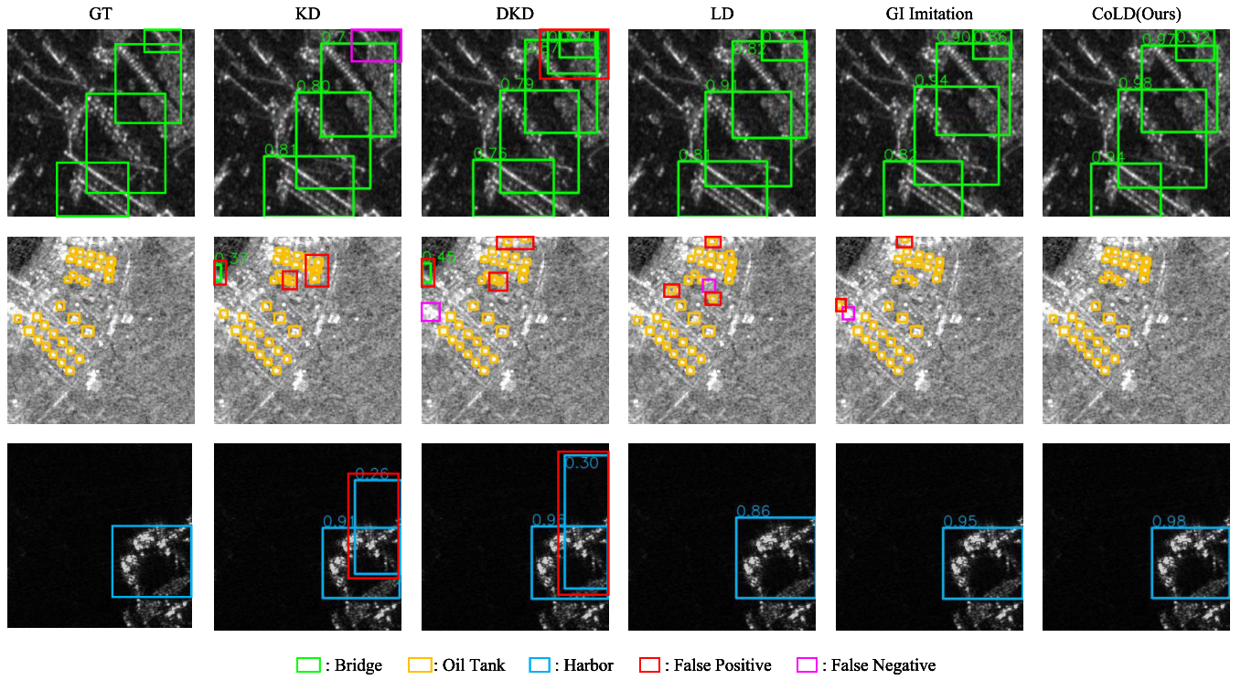
Fig. 5. Cross-modal KD strategies are visually compared. KD and DKD do not employ localization information, which leads to occasionally missed detections, while LD improves the results somewhat but falls short of GI Imitation. Our method is more accurate and has fewer missed detections according to the inference result. The red and purple boxes indicate false positive and false negative, respectively.
