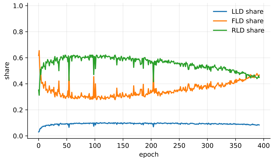
Full CCLKD: ATKD internal shares
