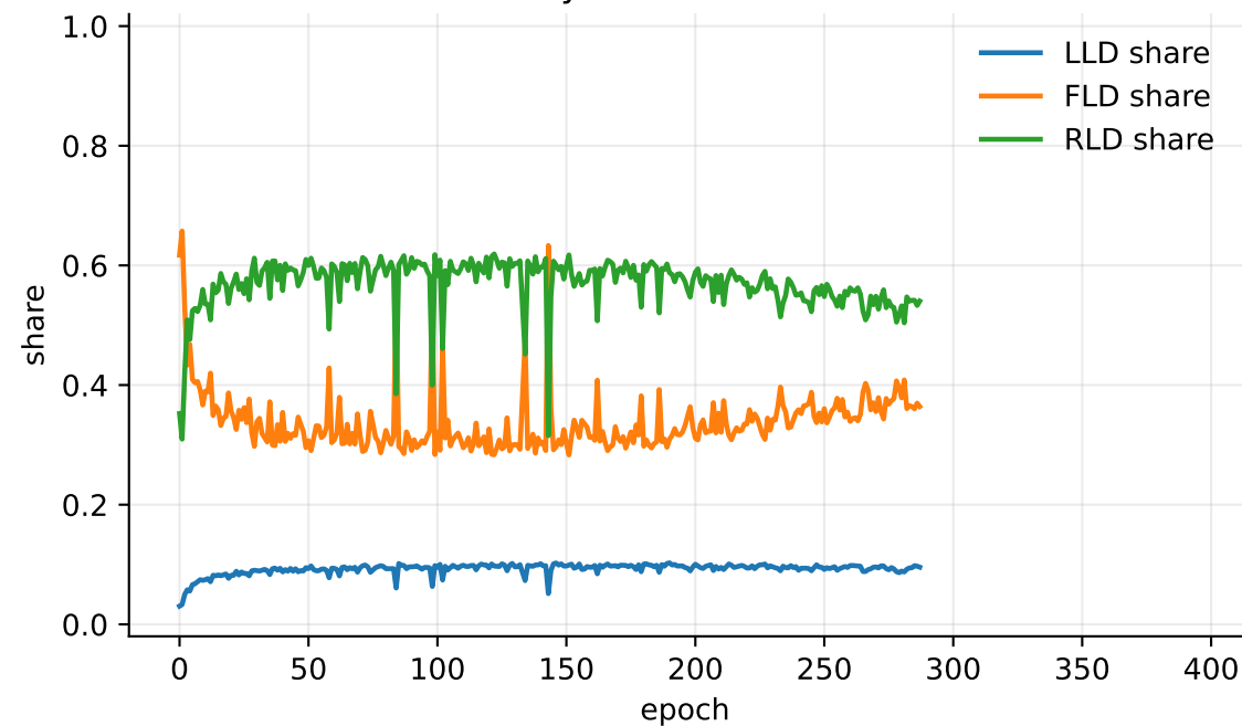
ATKD-only: ATKD internal shares
