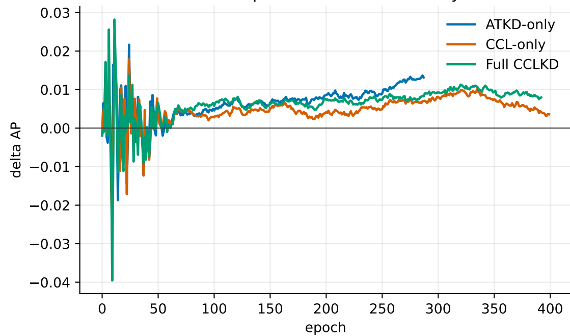
Same-epoch AP delta vs det-only
