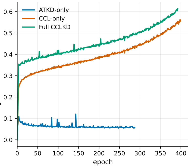
CCL loss
