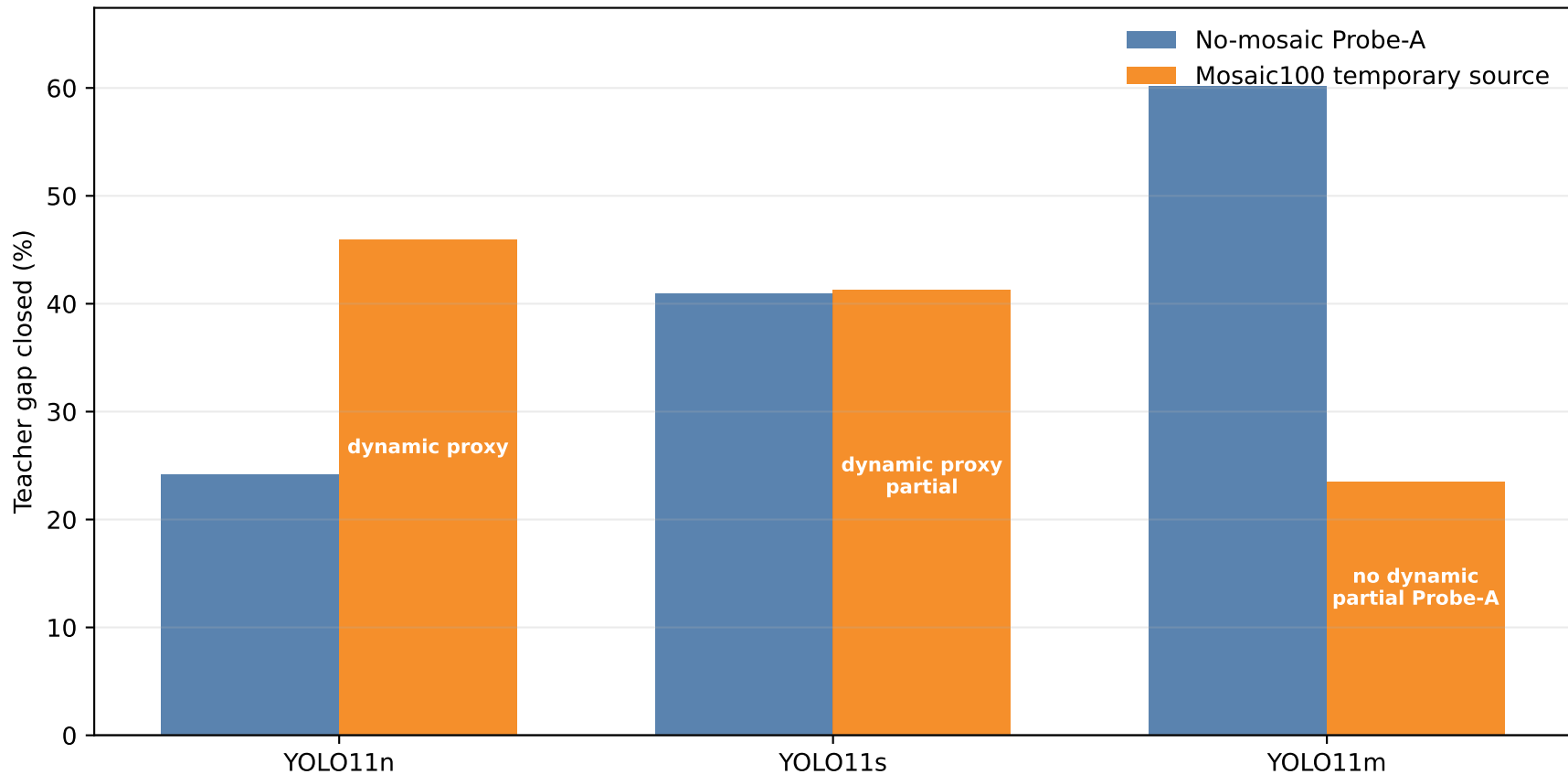
Teacher Gap Closed: No-mosaic vs Mosaic100 Temporary Source
