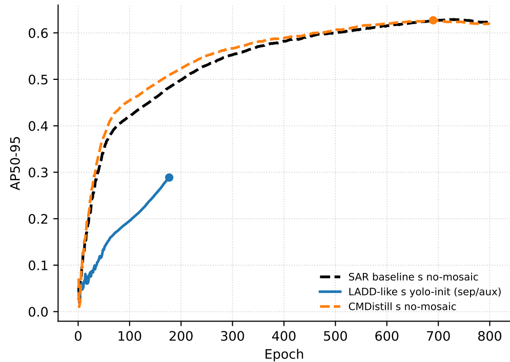
YOLO11s | formal no-mosaic
