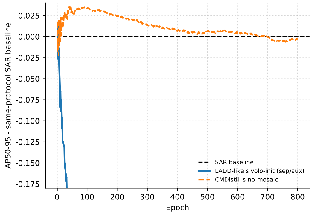
YOLO11s | formal no-mosaic
