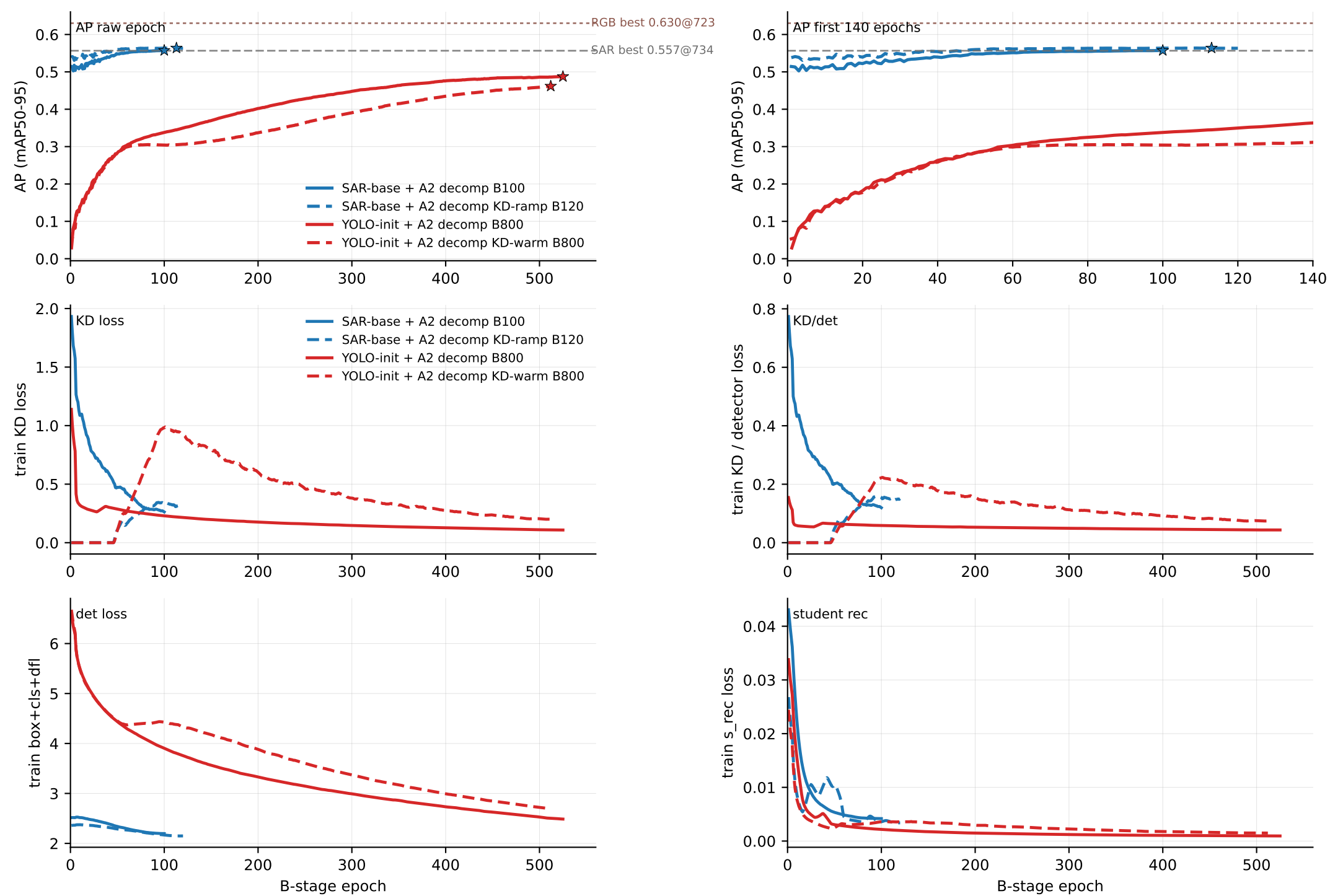
YOLO11n no-mosaic LADD-like split-load comparison. Blue = SAR-baseline detector init; red = YOLO-init detector. Solid = direct KD, dashed = KD warm/ramp. Note B100/B120 compressed schedules are not final B800-equivalent.
