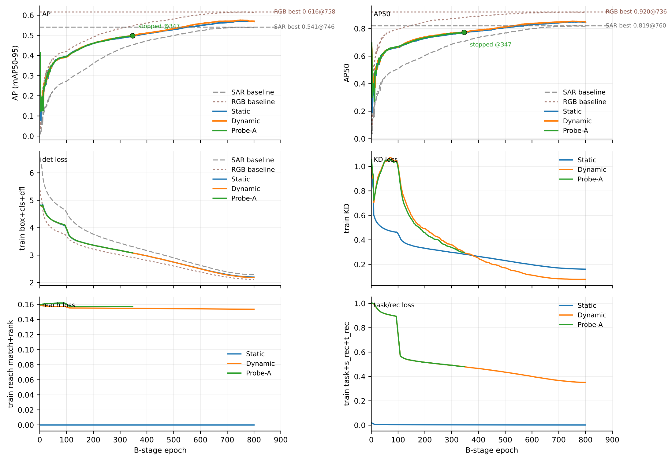
YOLO11n mosaic100 protocol. Thin dashed/dotted curves: same-capacity SAR/RGB baselines; horizontal lines: their best AP. Probe-A is the 4090 run interrupted at epoch 347; the green curve is short because the experiment has not been resumed.
