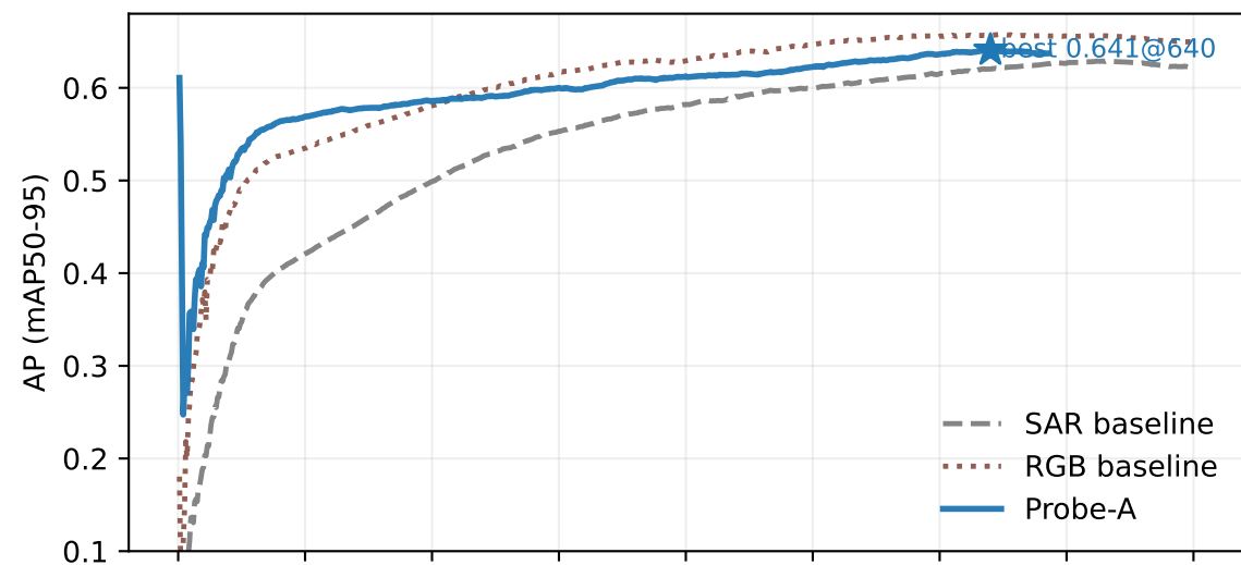
YOLO11s no-mosaic
