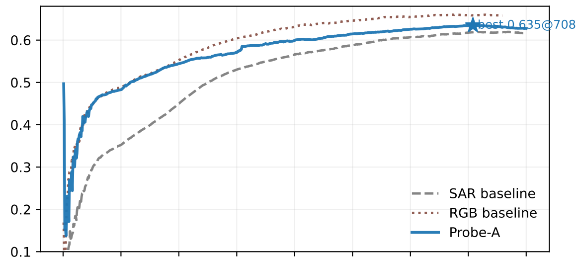
YOLO11s mosaic100
