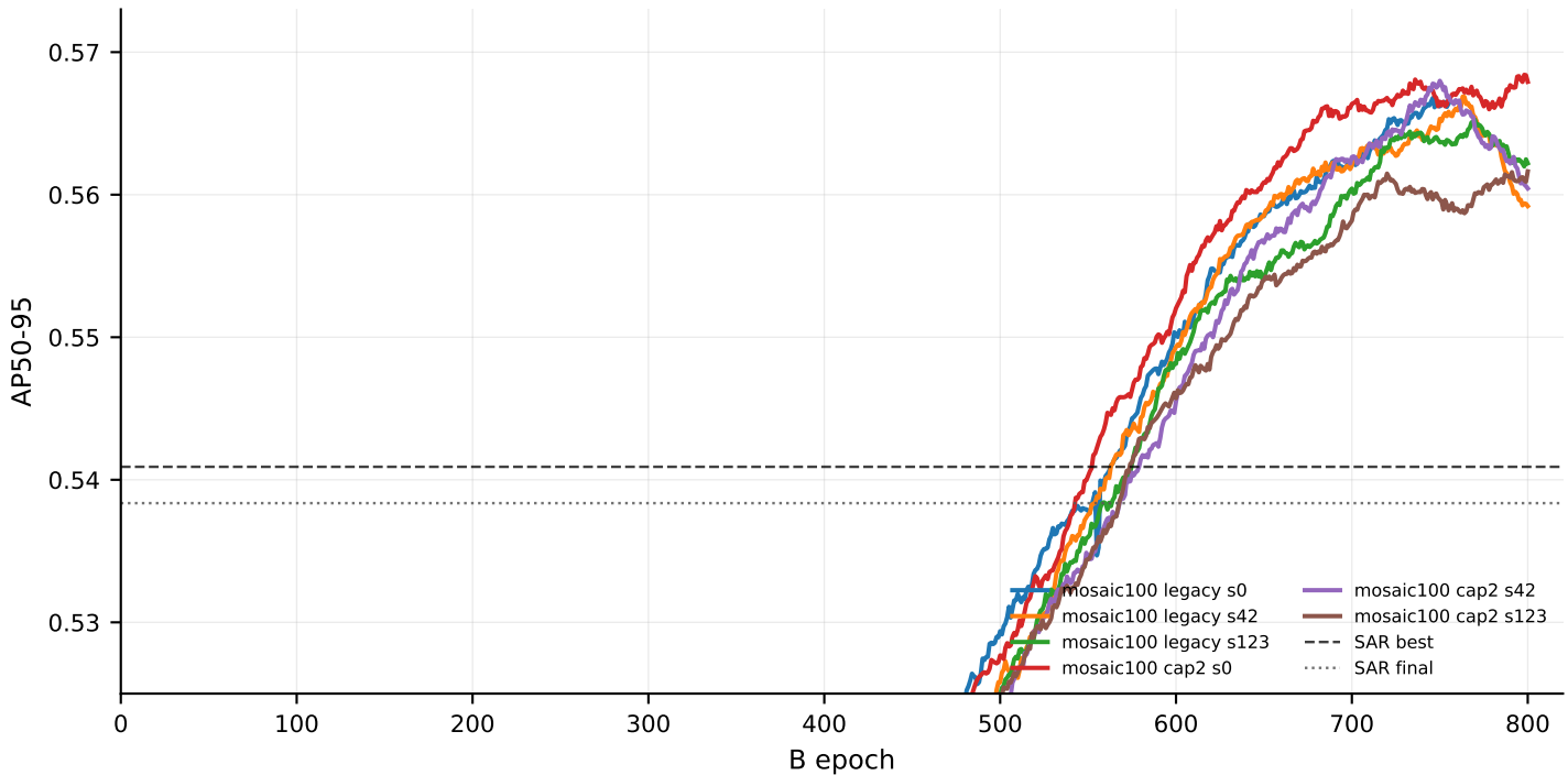
Old mosaic100/close@100 LADD curves
