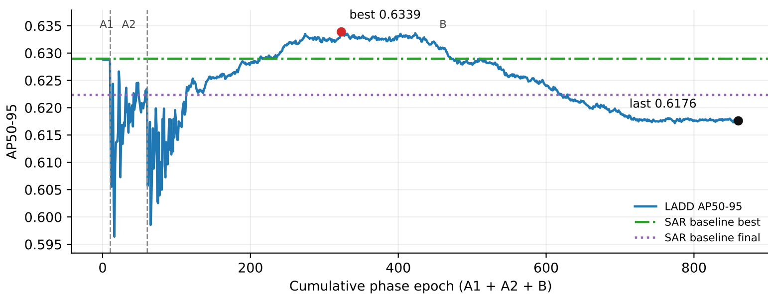
YOLO11s LADD phase AP curve
