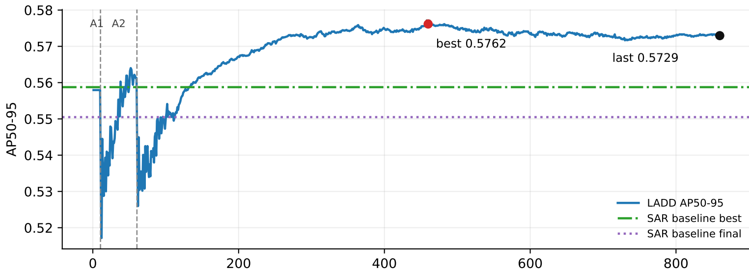
YOLO11s LADD phase AP curve
