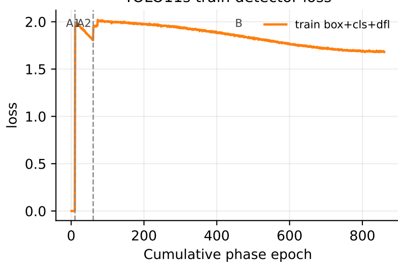
YOLO11s train detector loss
