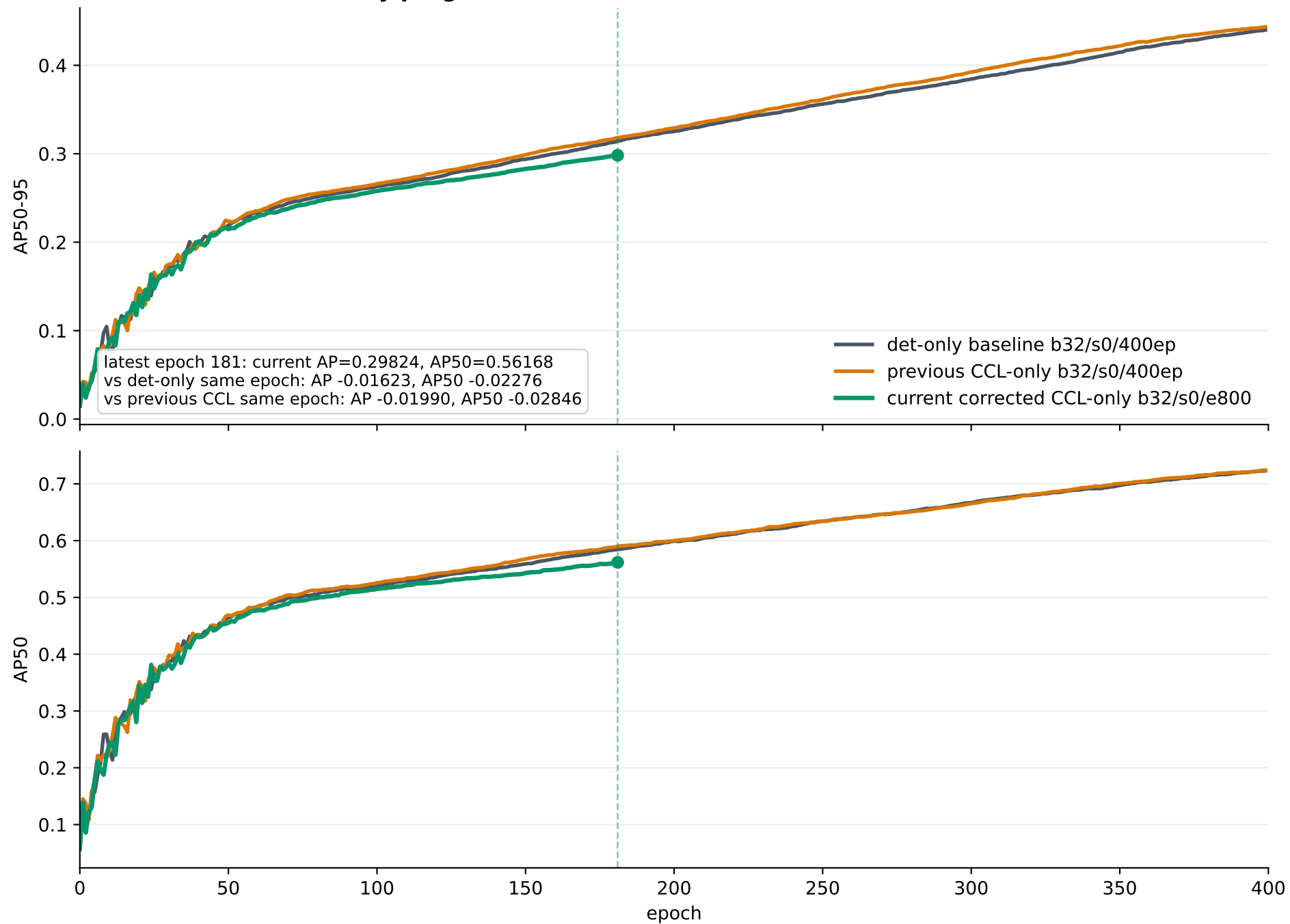
YOLOv5x CCLKD CCL-only progress vs baselines
