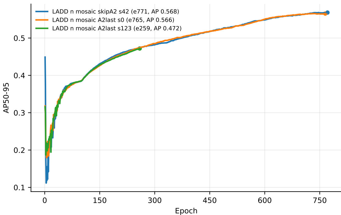
Mosaic LADD n runs
