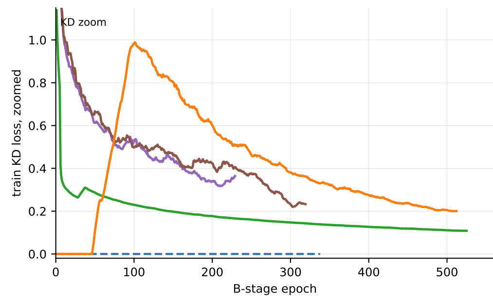
YOLO11n no-mosaic B800 restart diagnostics. N0/N1 are det-only controls, so KD loss is exactly zero; N2/N3/N4 show actual KD pressure.
