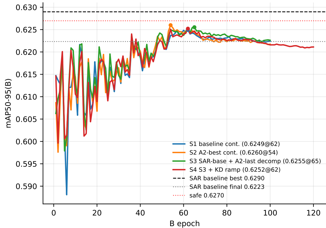
YOLO11s: B-entrance AP curves
