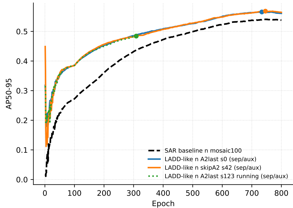
YOLO11n | mosaic100 / close@100
