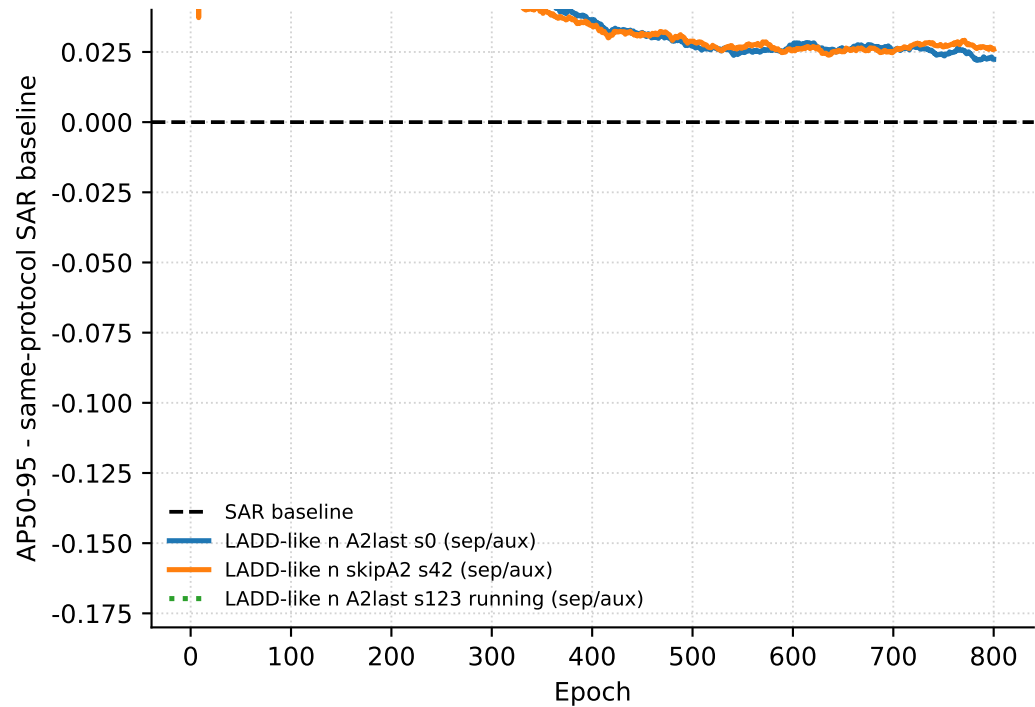
YOLO11n | mosaic100 / close@100
