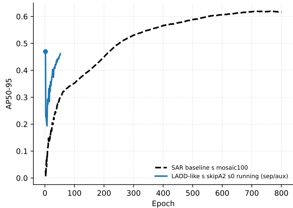
YOLO11s | mosaic100 / close@100
