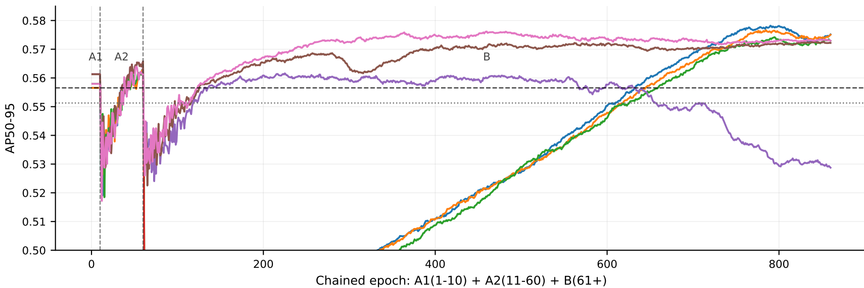
Formal no-mosaic YOLO11n A1->A2->B chain: zoom
