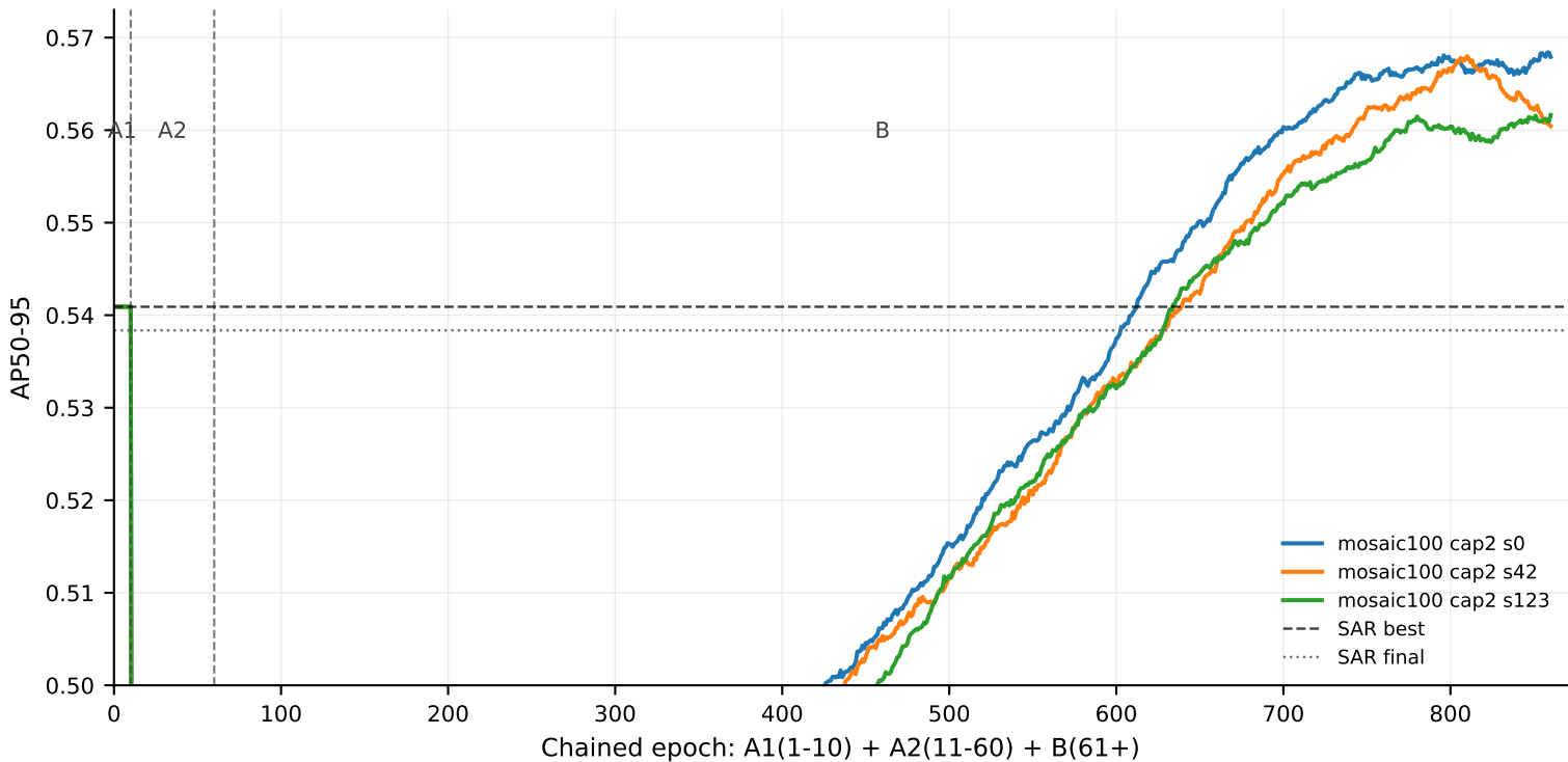
Mosaic100/close@100 YOLO11n A1->A2->B chain
