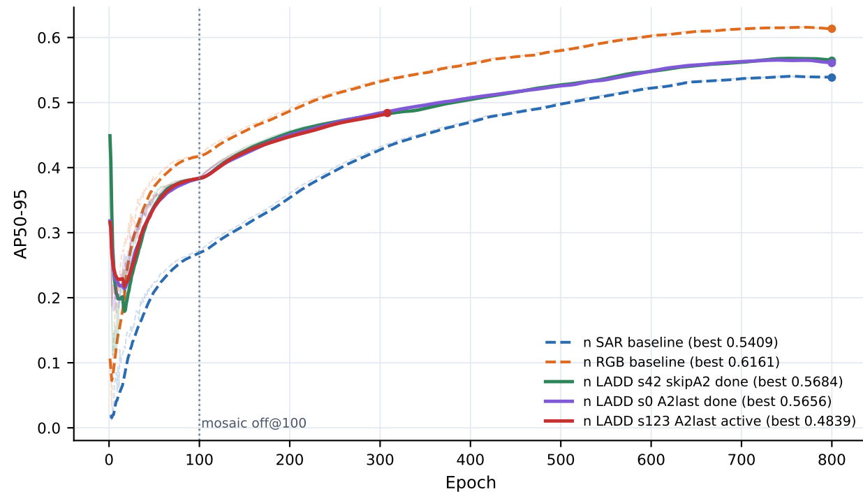
YOLO11m mosaic100 baselines currently running
