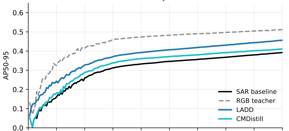
YOLO11s early AP50-95
