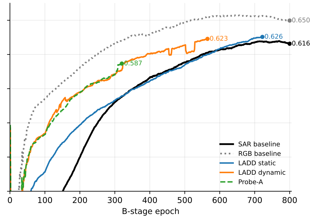
YOLO11s mosaic100 b64
