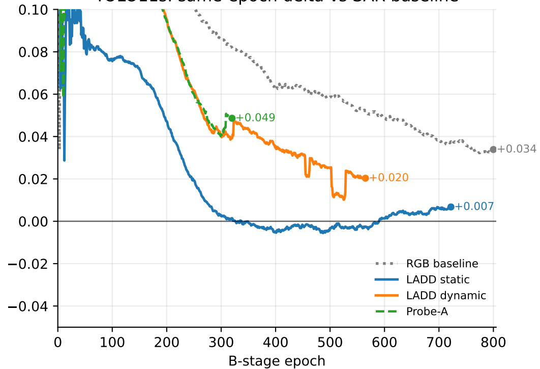
YOLO11s: same-epoch delta vs SAR baseline
