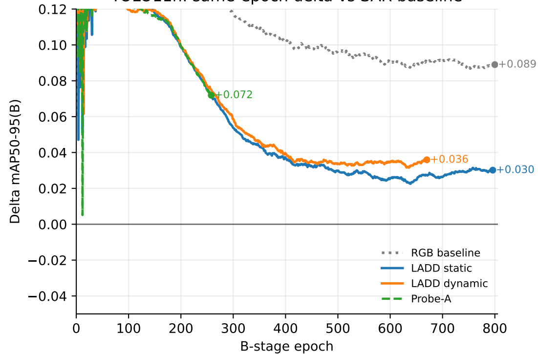
YOLO11n: same-epoch delta vs SAR baseline
