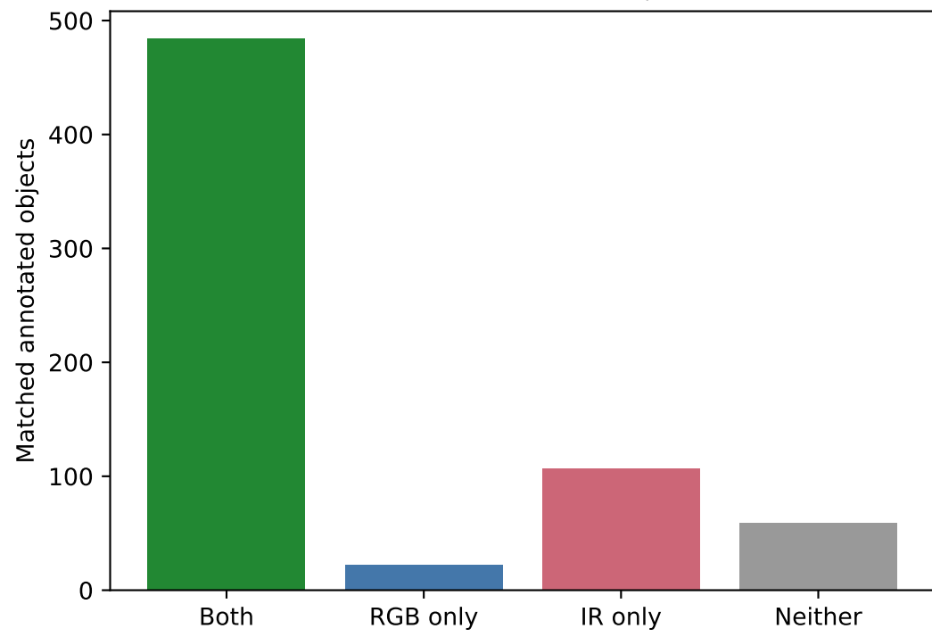
Baseline hits at conf 0.25, IoU 0.5
